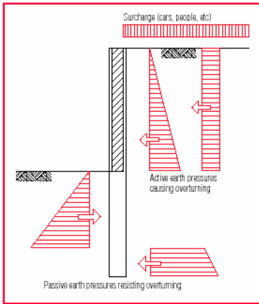
Figure 2 Piled wall
