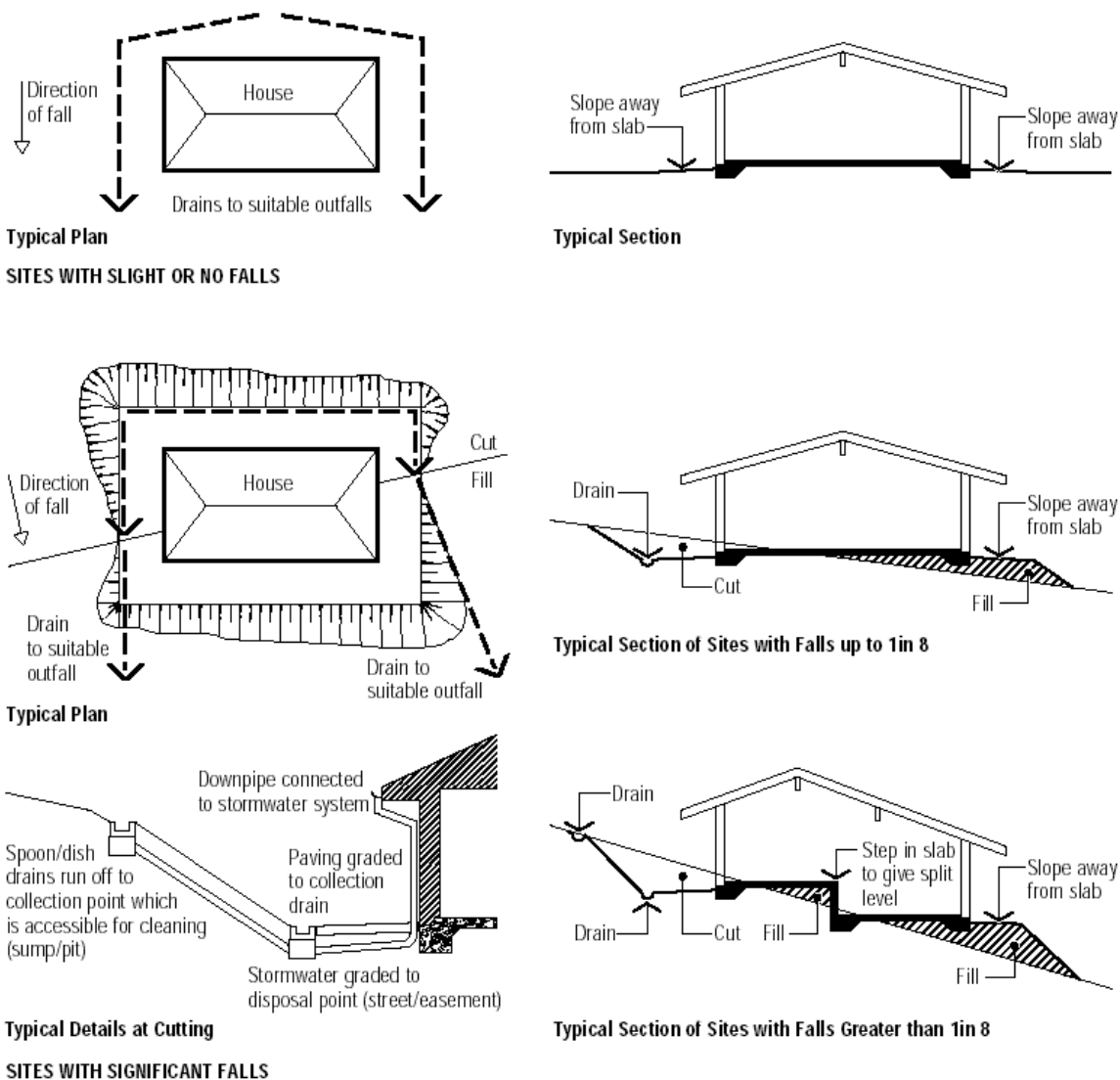
Figure 4.10 Stormwater drainage
