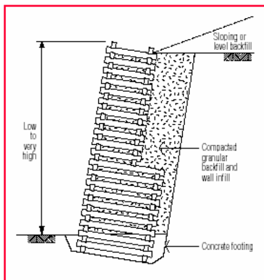
Figure 6 Crib wall
