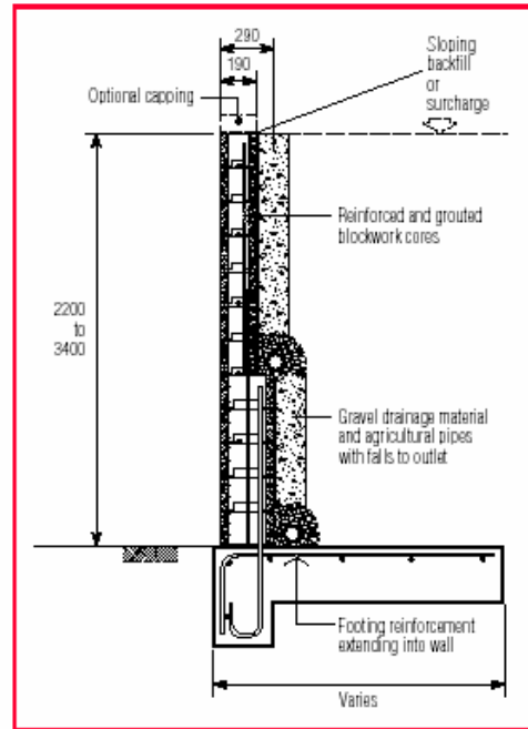
Figure 3 Concrete masonry
