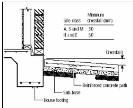
Figure 4.9 Minimum crossfall of paving for given site classifications
