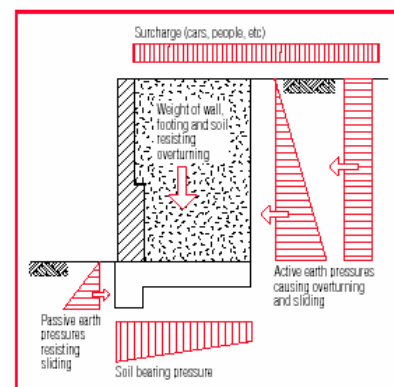
Figure 1 Gravity wall
