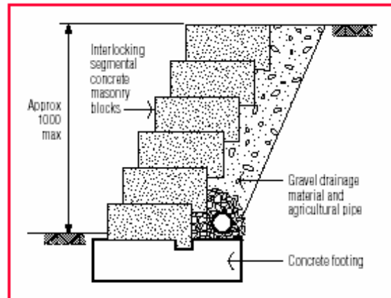
Figure 4 Segmental block
